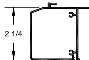
2 1/4" CLAD SUBSILL EXTRUSION
