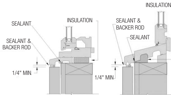
FIG. 16: CASEMENT SILL
